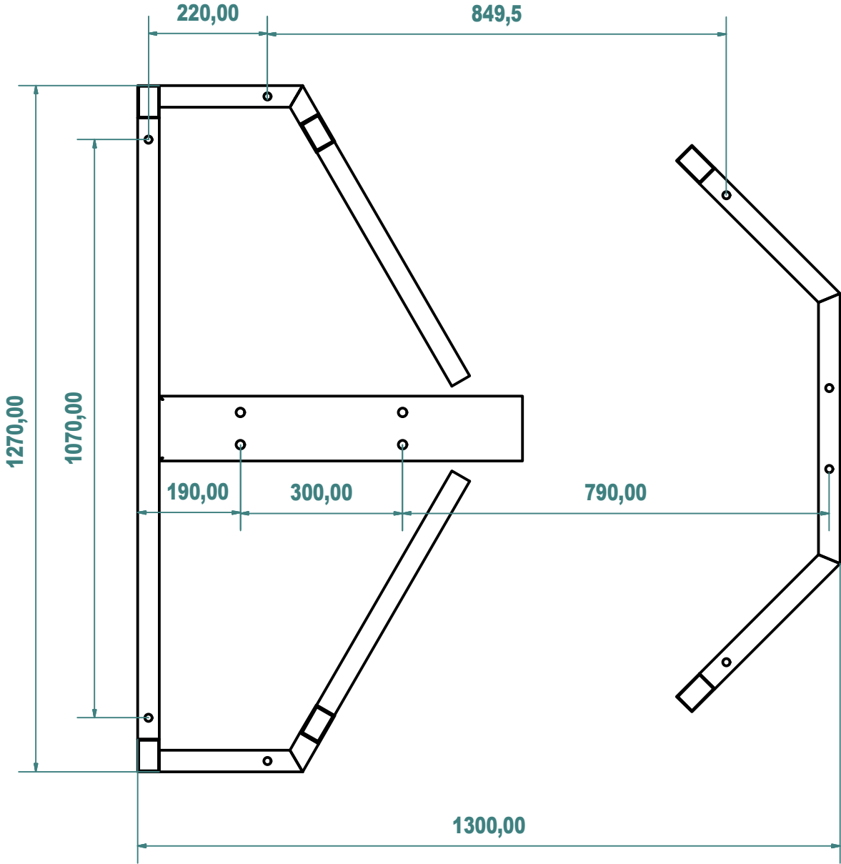
FULL HEIGHT TURNSTILE TOP VIEW
