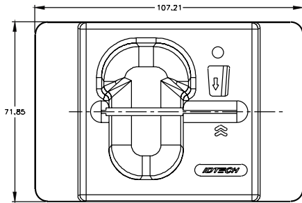
Large Flush Mount Bezel Recommended Cutout
