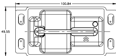
Large Standard Bezel & Recommended Cutout
