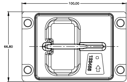
Metal Flush Mount Bezel & Recommended Cutout
