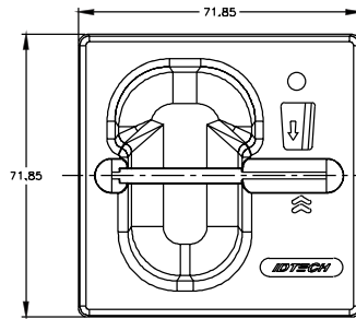
Standard Flush Mount Bezel Recommended Cutout
