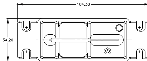
Standard Bezel & Recommended Cutout
